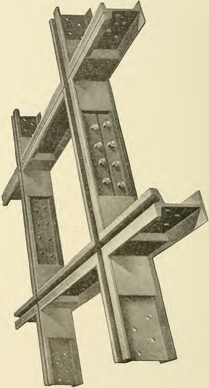
Fig. 239. Grooved Rail Right-Angled Cross
